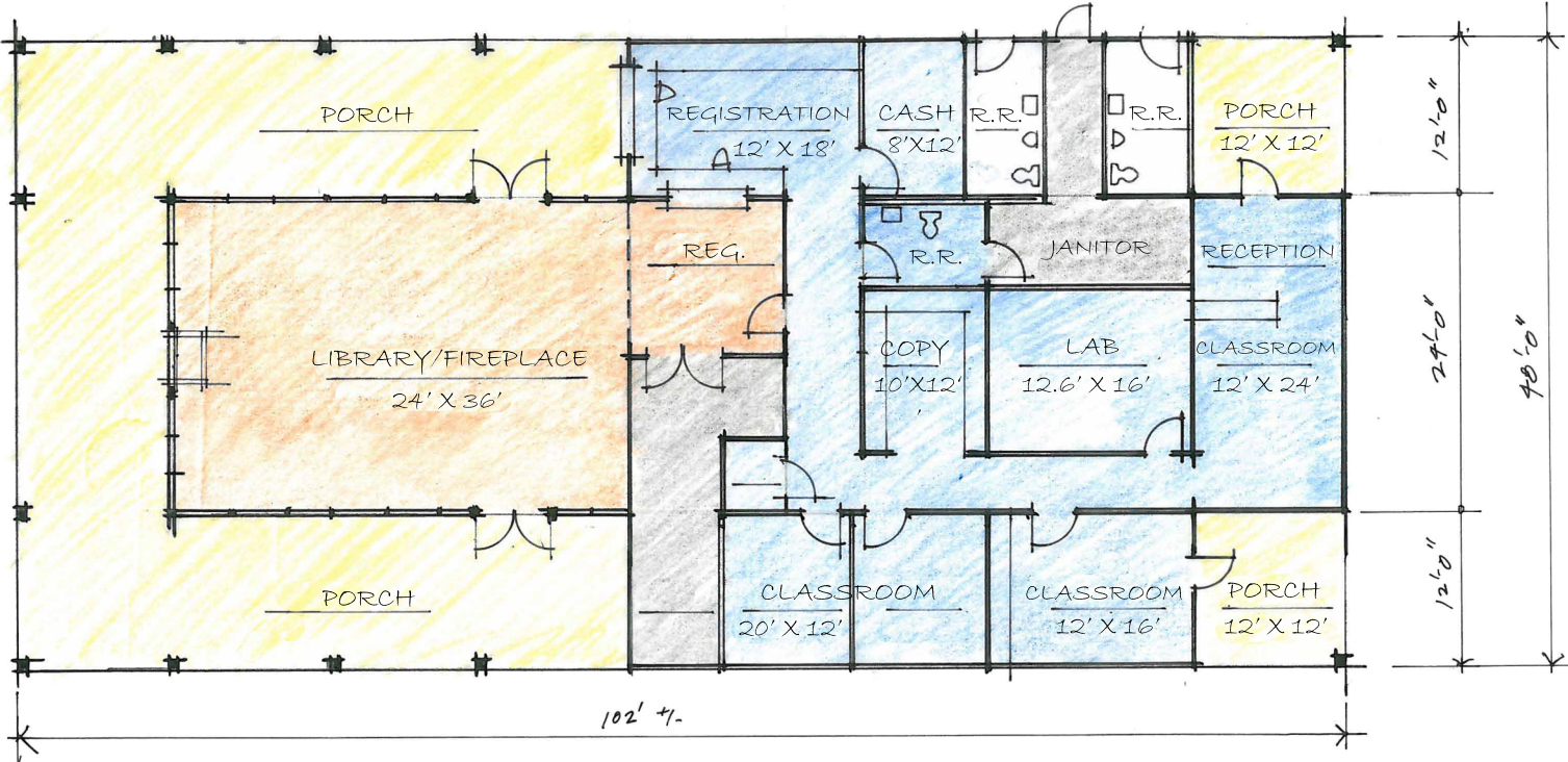
EDUCATION CENTER FLOOR PLAN 1728 SF - PORCHES : 3264 # · INTERIOR S.F. 1/8" = 1' 0"
