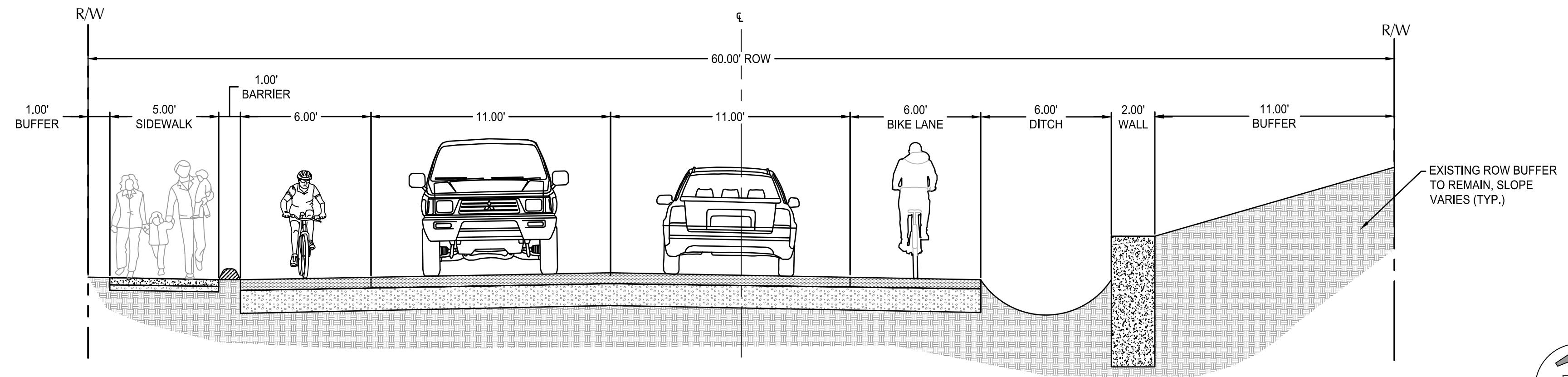
OPTION 2 SECTION REDUCED WIDTH SCALE: 1" = 4'
