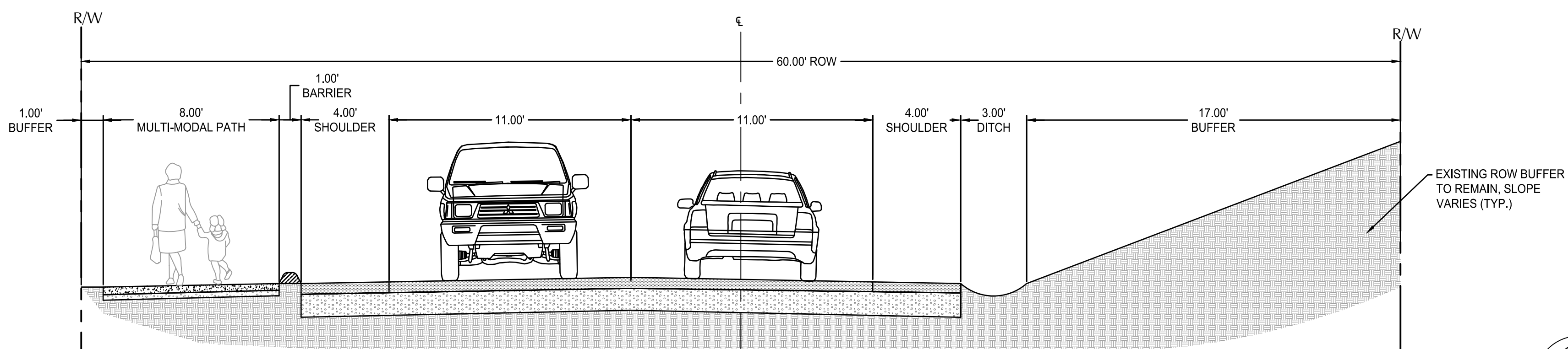
OPTION 1 SECTION REDUCED WIDTH SCALE: 1" = 4'
