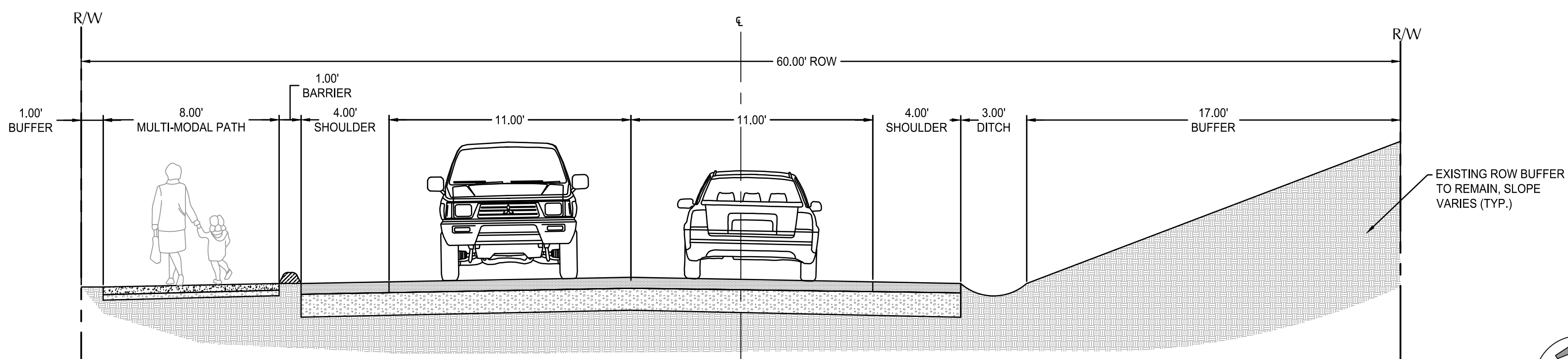
OPTION 3 SECTION REDUCED WIDTH SCALE: 1" = 4'
