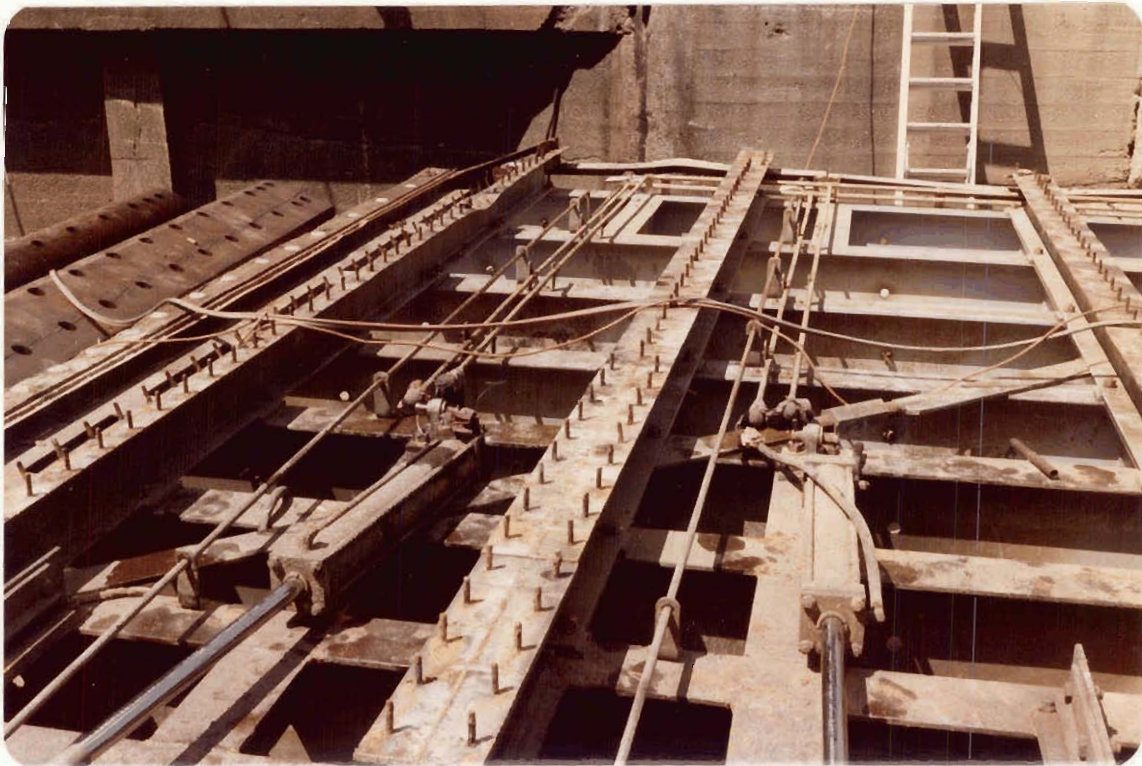
Frame (6) 4 May 82 Gate No. 1 Left Leaf
