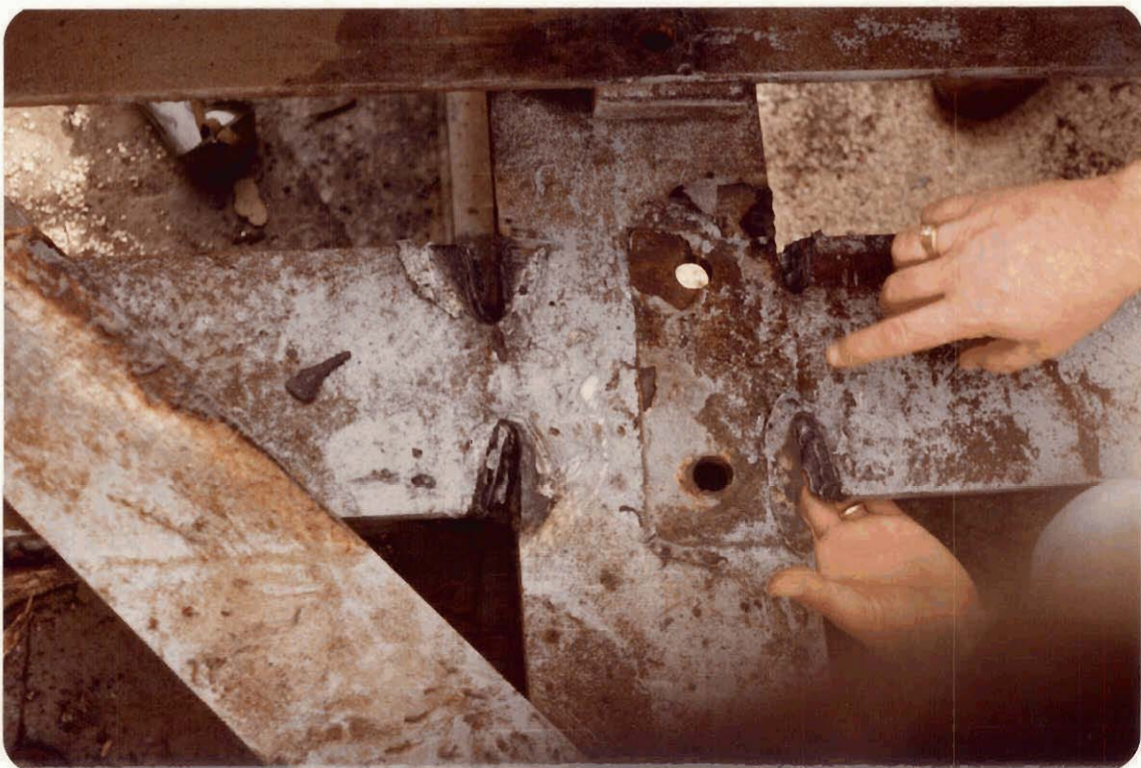
Frame (11) 5 May 82 Gate No. 1 Left Leaf Airgauged cracks
