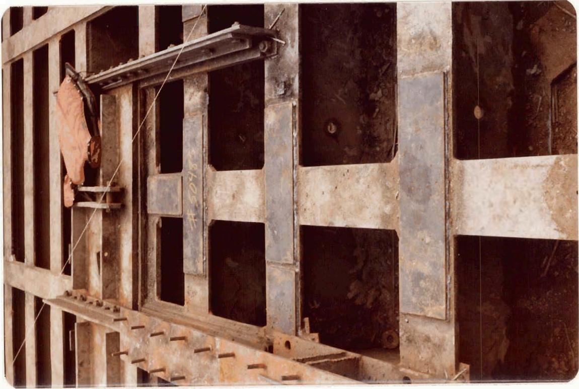
Frame 2A - Left Leaf - Flange Repair Plate May 11, 1982
