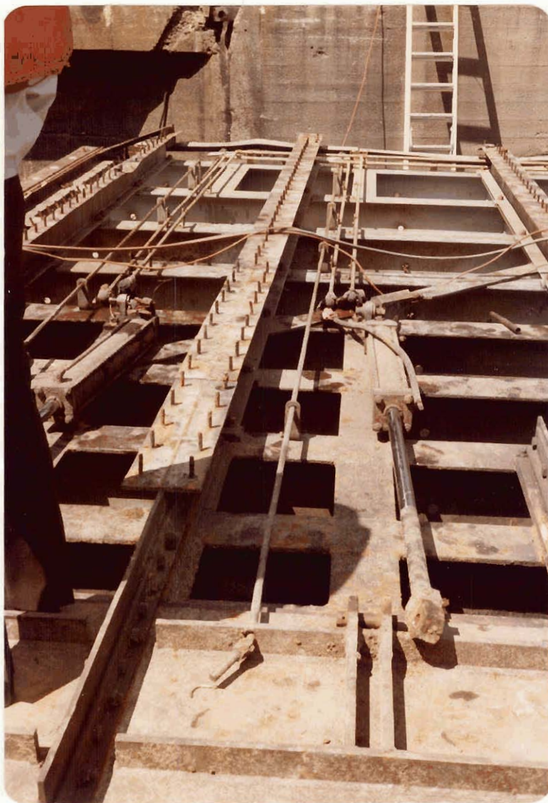
Frame (4) Gate No. 1 4 May 82 Left Leaf
